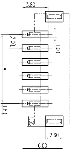
PCB LAYOUT
